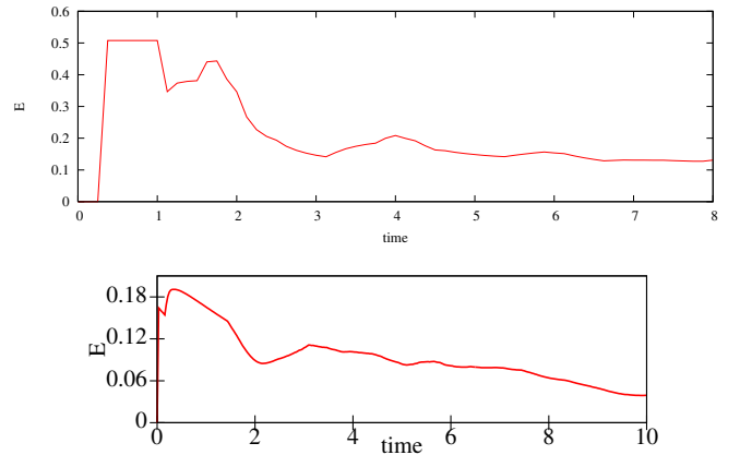
Fig. 6. Tracking results with MICA-2 acoustic sensors (top) and the corresponding simulation (bottom). The following simulation parameters are used: grid separation distance 0.4 m = 1.0 unit, sensing range R = 1.5 unit, R_e = 0.2R , and target velocity v=0.5 unit/sec.
