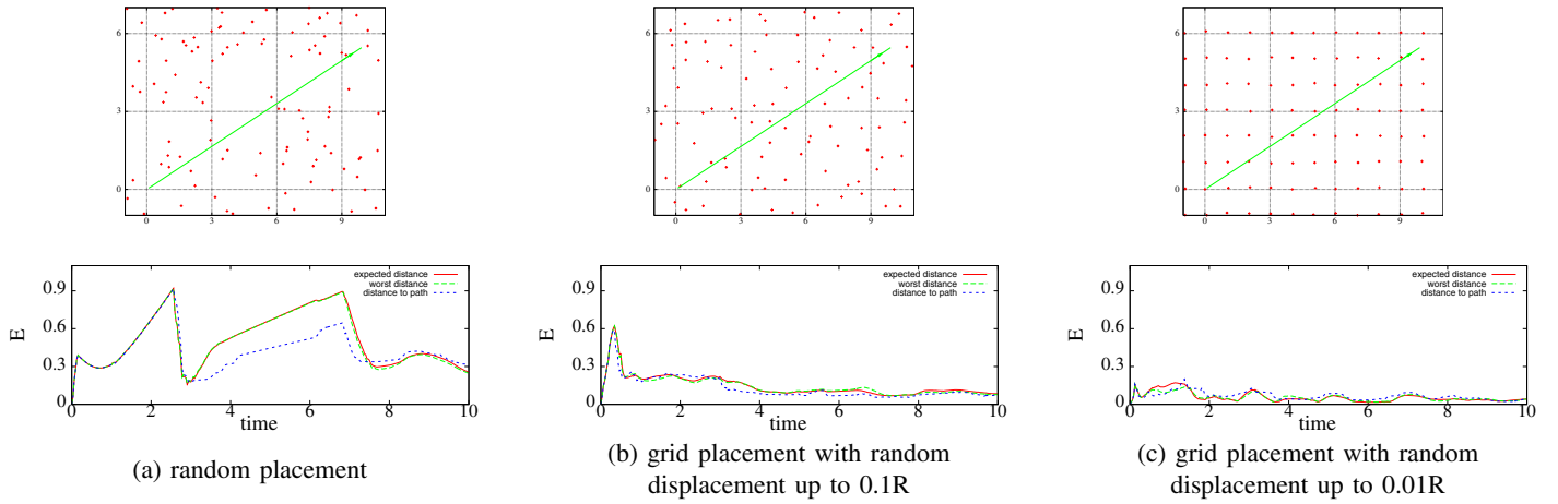
Fig. 11. Three different placements and the respective tracking performance. Density = 1.0, N = 900 , R = 1.0 u , R_e = 0.2R . Average of 100 simulation runs.
