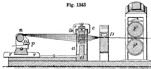
Cloth-Folding Machine.
