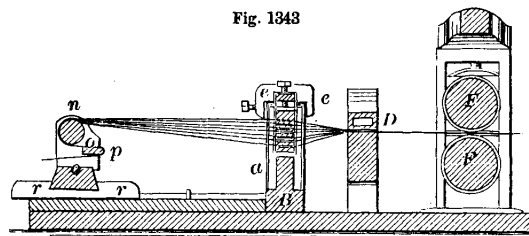
Cloth-Folding Machine.
