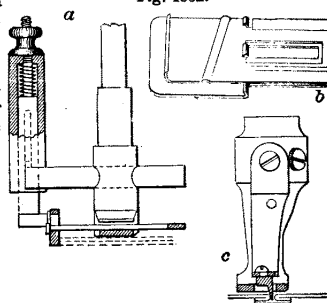
Sewing-Machine Gages.
