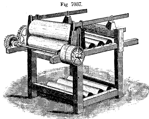
Warp-Dyeing Machine.
