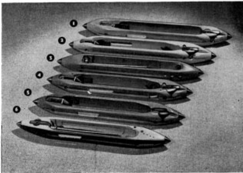
BELOW. (1) Shuttle for automatic wool loom. (2) Shuttle for automatic worsted loom. (3) Shuttle for plain worsted loom. (4) Shuttle for automatic cotton loom (equipped with brass threader). (5) Shuttle for automatic cotton loom (equipped with cast iron threader). (6) Shuttle for silk or rayon loom (equipped with Paterson tension and fibre covered on one side).
