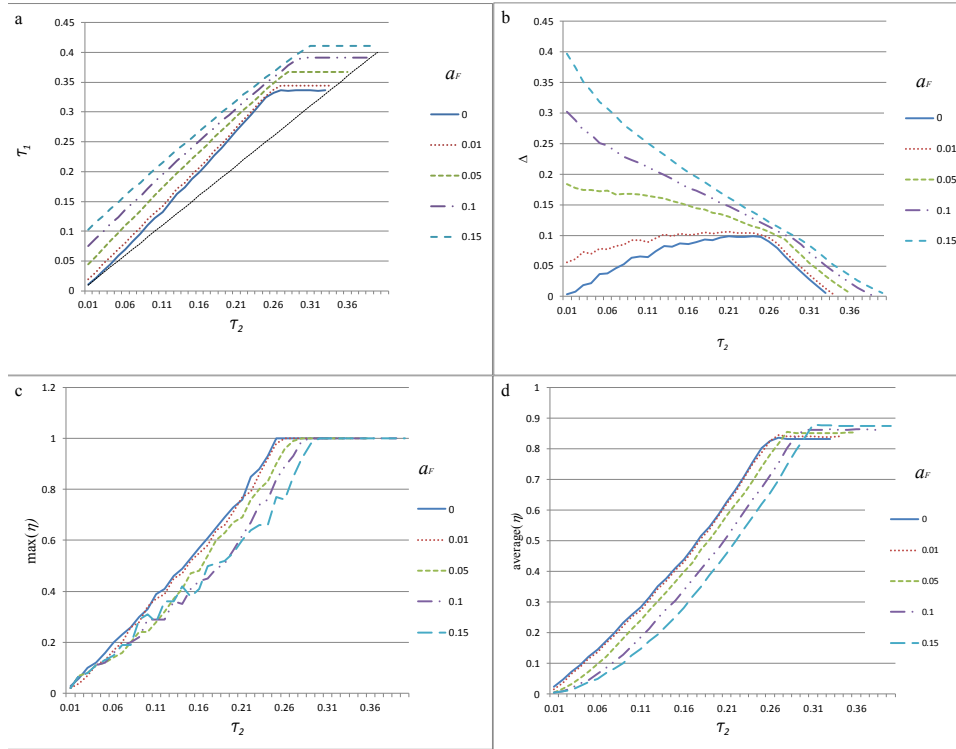
Figure 7. Simulation results. For different \alpha_F values, (a) presents the maximum achieved \tau_1 threshold given \tau_2 . (b) presents the delta capacity, which is equivalent to the achievable communication rate. (c-d) present the maximum jammer activity and the average jammer activity versus \tau_2 , respectively.
