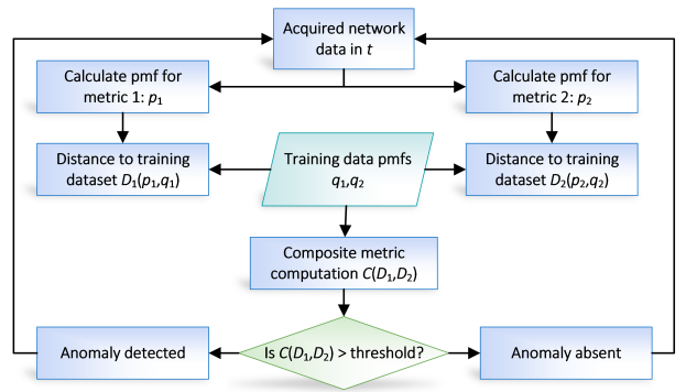
Figure 6: Flowchart of the anomaly detection process
