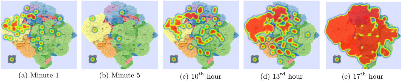
Figure 8: Heat maps for CodeRed Worm propagation. (a,b) Worm initially spreads; (c) reaches several countries at once; (d) propagates to several ASes within the same country; and (e) attains the peak of activity in (e).
