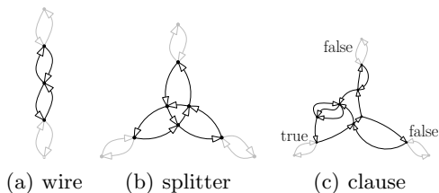
Fig. 7. The gadgets used in the reduction; gray edges show how adjacent gadgets are connected.
